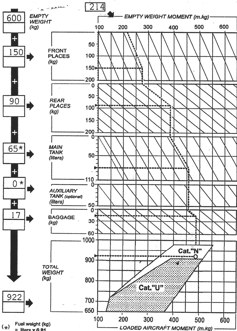
Figure 6-1 Weight and Balance
